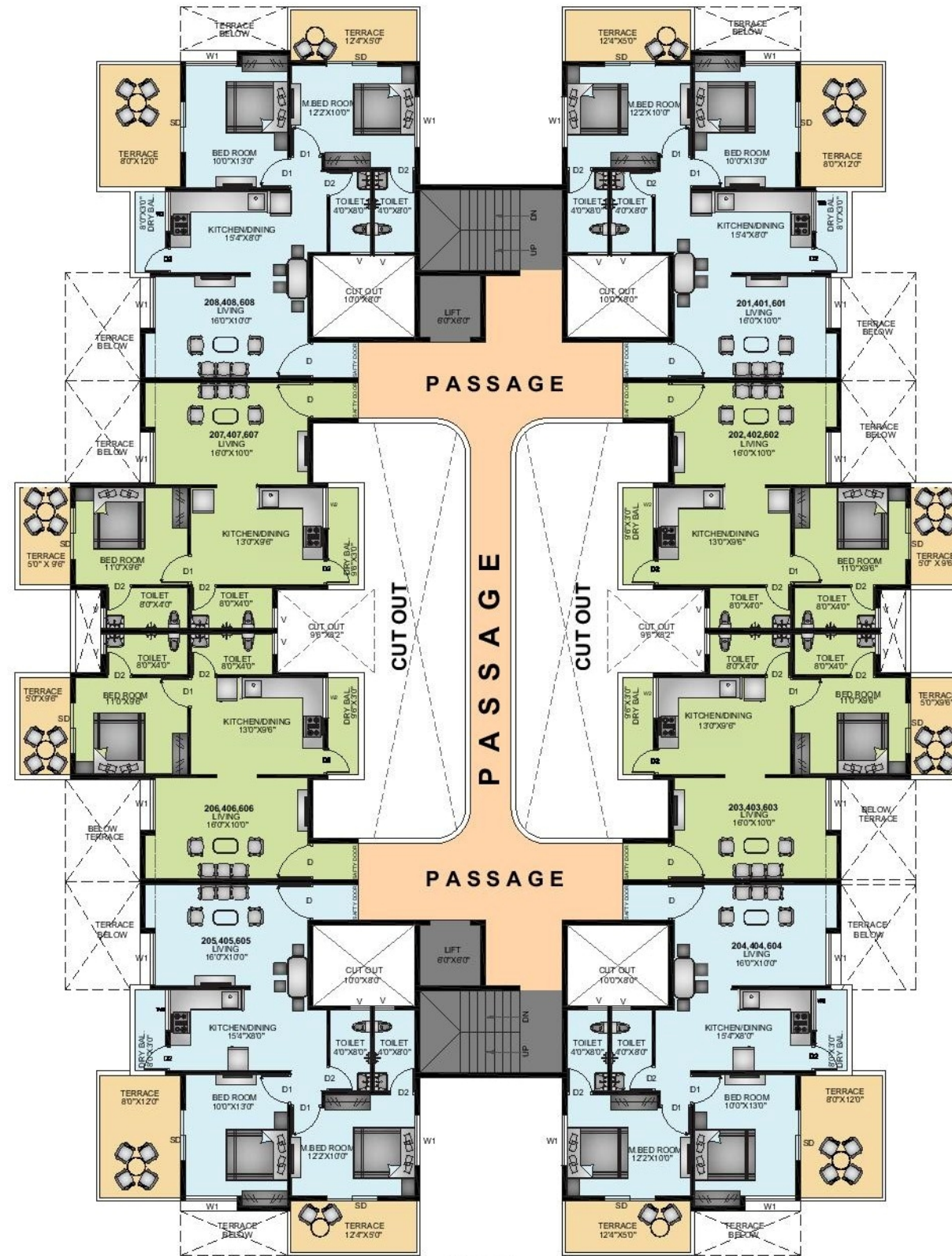
WING C 2nd,4th,6th FLOOR PLAN
