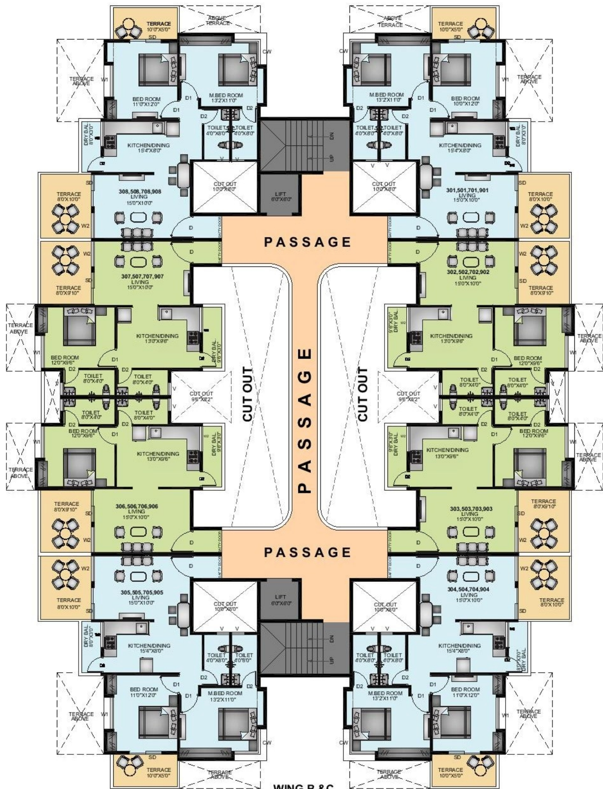
WING B & C 3rd,5th,7th & 9th FLOOR PLAN
