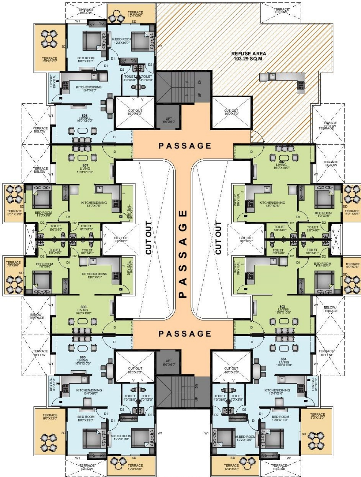
WING B & C 8TH FLOOR PLAN
